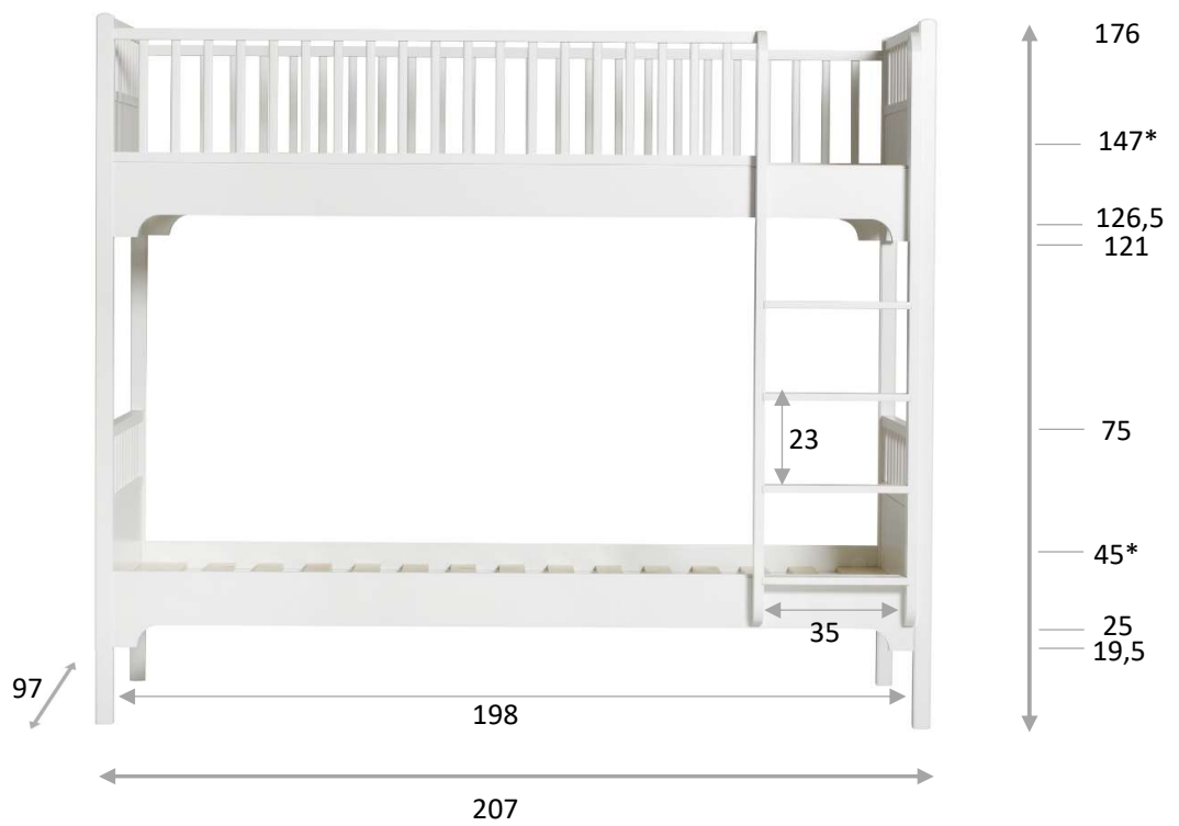
Classic Bunk bed 021219
